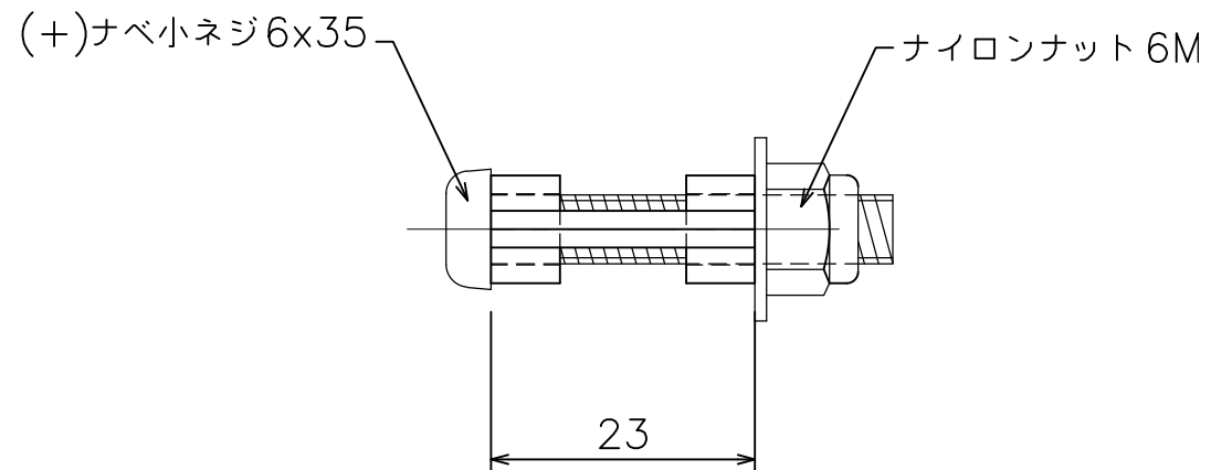
U継金具 (90T91)
